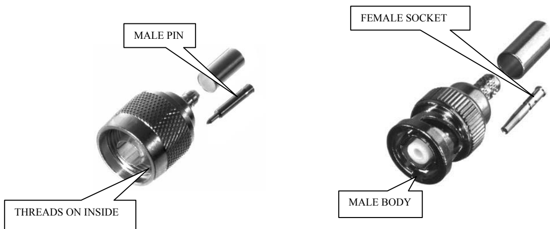
(N-Male Connector)
