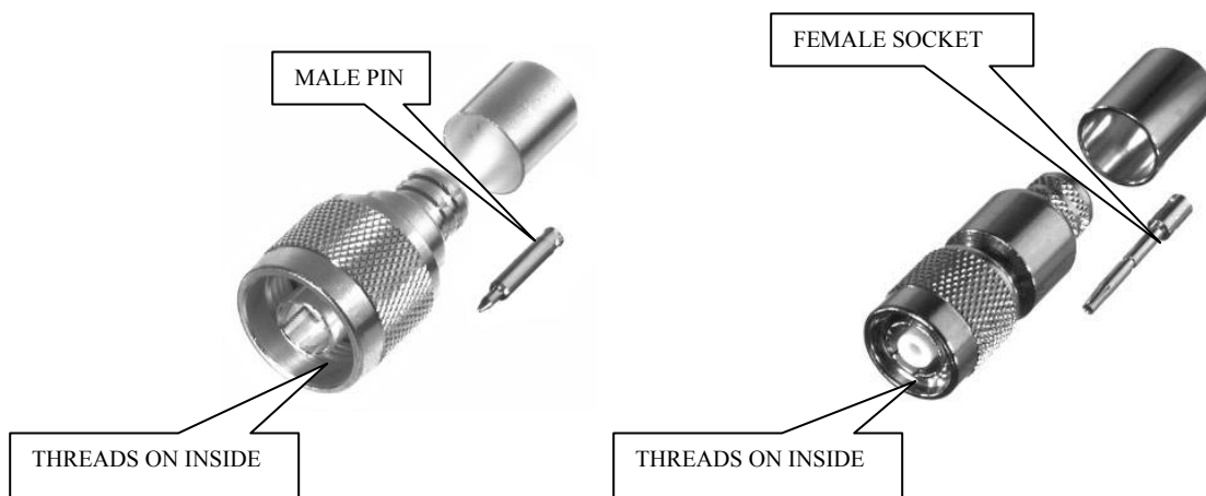
(N-Male Connector)
